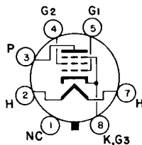
BOTTOM VIEW BASING DIAGRAM JEDEC TAC
