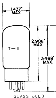
GLASS BULB SHORT INTERMEDIATE SHELL 7 PIN OCTAL A7-47 OUTLINE 11-1
